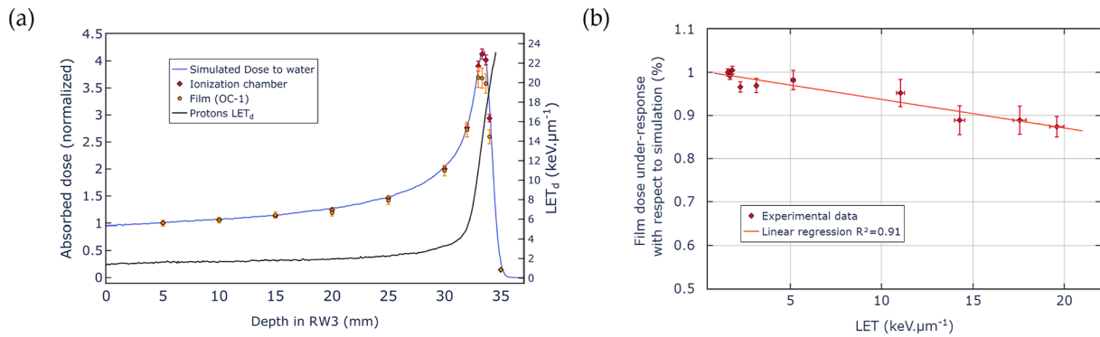
Fig. 4. (a) In-depth measurement of the quenching effect of OC-1 films in RW3 slabs, (b) linear relationship between film under-response and proton LET d in RW3.
