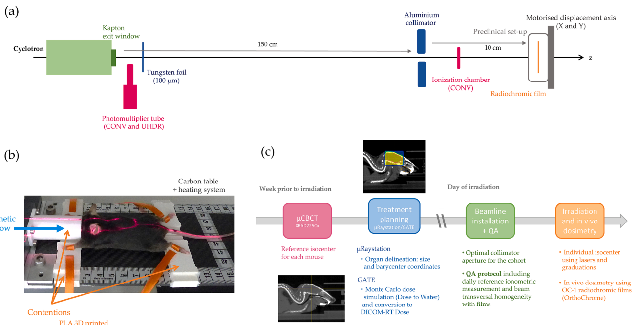
Fig. 1. (a) Schematical view of the ARRONAX irradiation beamline; (b) Photograph of the positioning system (3D-printed immobilization system and graduations); (c) Workflow diagram.
