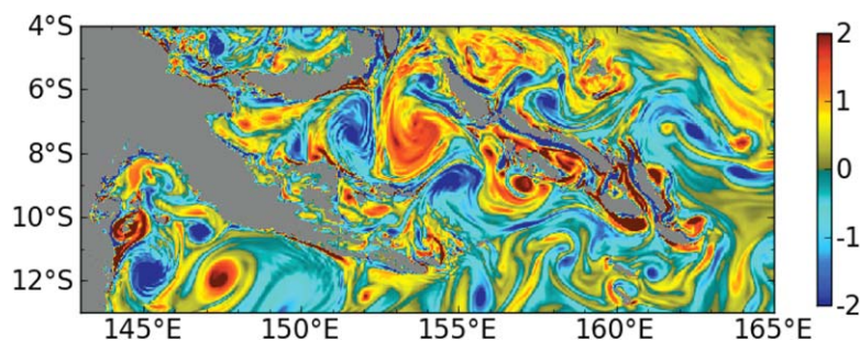
Figure 6. Potential vorticity at 20 m depth on 31 March 1995 from the 1/36° resolution NEMO Solomon Sea model simulations (full PV; unit is 10^{-7} \text{ kg m}^{-4} \text{ s}^{-1} ).
