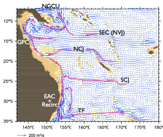
Figure 7. 0–1000 m transports estimated from the relative geostrophic velocity from CARS climatology [Ridgway et al., 2002] combined with mapped average absolute velocity at 1000 m from Argo float drift. The main currents are indicated as in Figure 2. From Kessler and Cravatte [2013a].
