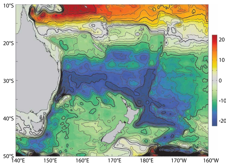
Figure 4. OFAM3 model full-depth transport streamfunction [Oke et al., 2013]. Contour interval is 1 Sv ( 1 \text{ Sv} = 10^6 \text{ m}^3 \text{ s}^{-1} ).
