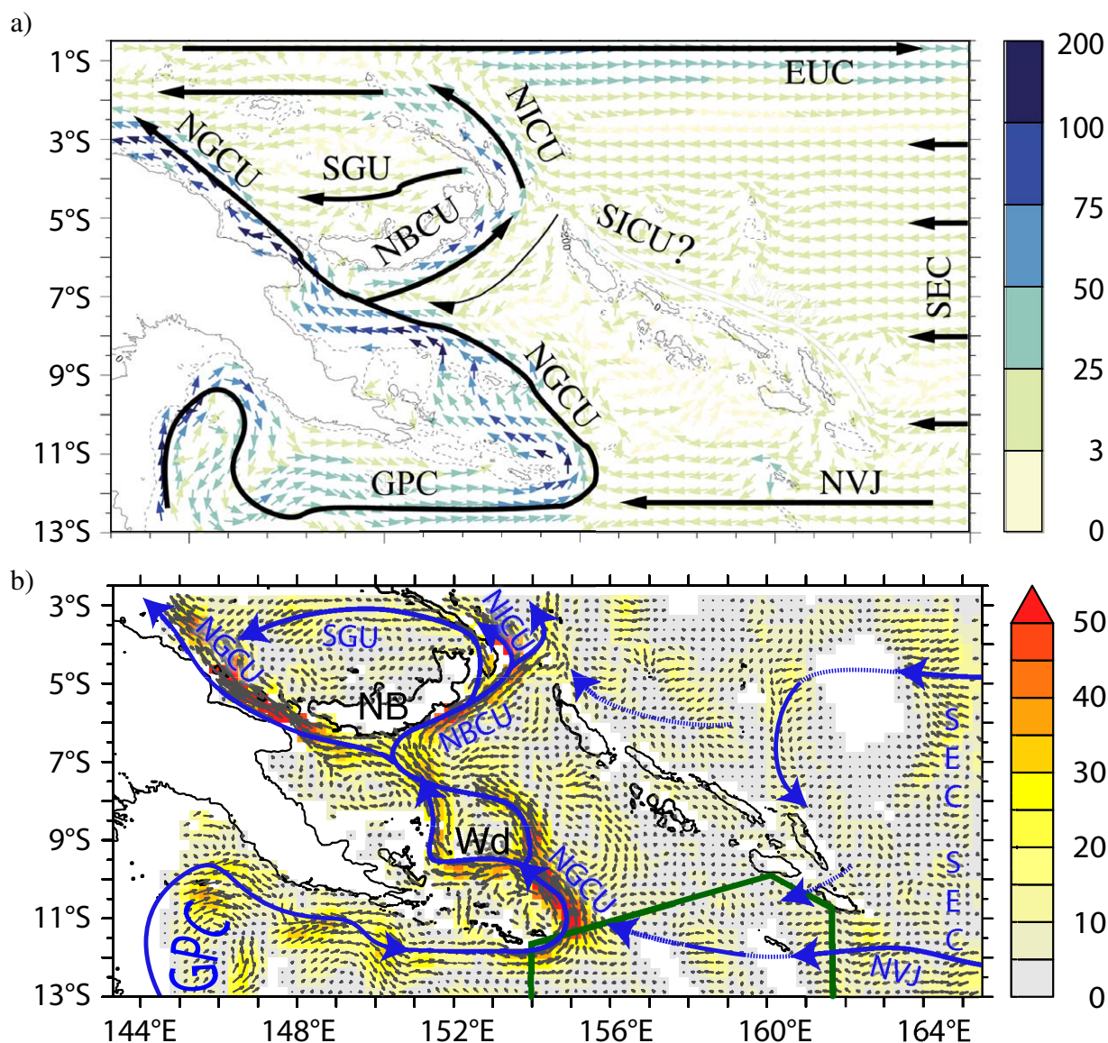
Figure 12. Mean circulation in the Solomon Sea thermocline. (a) From the 1986–2004 mean of a 1/12° simulation, and vertically integrated from the isopycnal surfaces \sigma_\theta = 24.0 to 26.5 \text{ kg m}^{-3} [adapted from Melet et al. , 2010a]. (b) From a climatology of shipboard-ADCP data, averaged over the 100–300 m layer adapted from Cravatte et al. [2011]. In (b), the green straight lines locate the 2007 oceanographic cruise track (see text) New Britain (NB) and the Woodlark Archipelago (Wd) are indicated, as well as the main currents as on Figure 2, as well as St George Undercurrent (SGU); New Britain Coastal Undercurrent (NBCU); and an hypothetical Solomon Island Coastal Undercurrent (SICU; see text).
