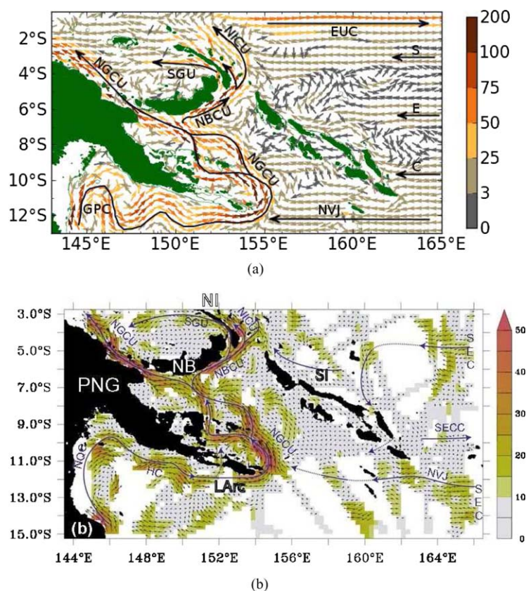
Figure 3. Mean circulation over 1993–2007 in the Solomon Sea integrated in the thermocline over \sigma = 24\text{--}26.5\text{ kg/m}^3 (in \text{m}^2\text{s}^{-1} ), (a) from the 1/36^\circ model and (b) from SADC data (in \text{cm s}^{-1} ) [Cravatte et al. , 2011].
