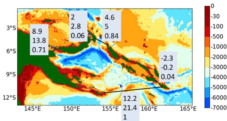
Figure 8. Model transport estimates in the main Solomon Sea straits (Vitiiaz Strait, St George's Channel, Solomon Strait, and Indispensable Strait) and through the southern section: 0–300 m transport, full depth transport (Unit: Sv). The third numbers show the correlations between the southern section transport and the thermocline transports within the corresponding strait. The blue arrows indicate the direction of the transport.
