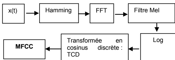
Figure 1 – Algorithme de calcul des coefficients MFCC
