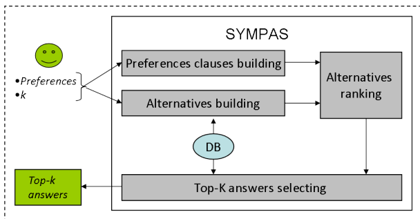
Figure 1: SYMPAS architecture
