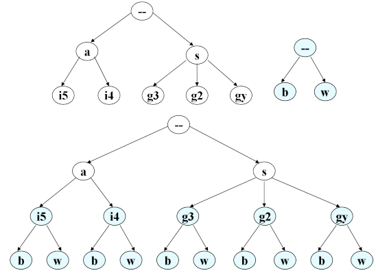
Figure 2: Preference representation
