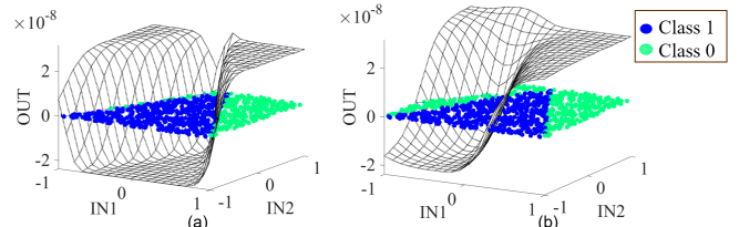
Figure 1: (a) Model Learned via Chip-in-the-Loop Training, (b) Model Ported to Same HW Resources on Identical Chip.
