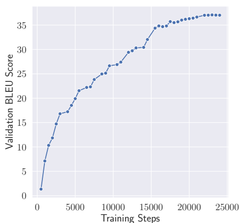
Figure 5: Tracking Prot2Text BASE BLEU Score Progression on Validation Set Across Training Iterations. Higher is better.
