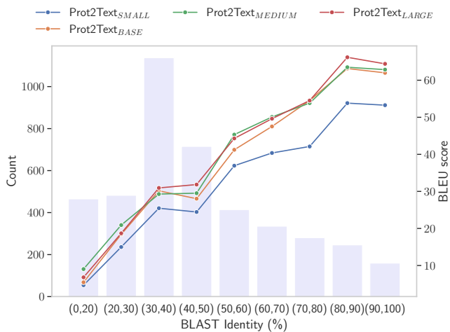
Figure 2: The test BLEU score for Prot2Text models as a function of the percentage identity using BLAST hit between the test and the train sets.
