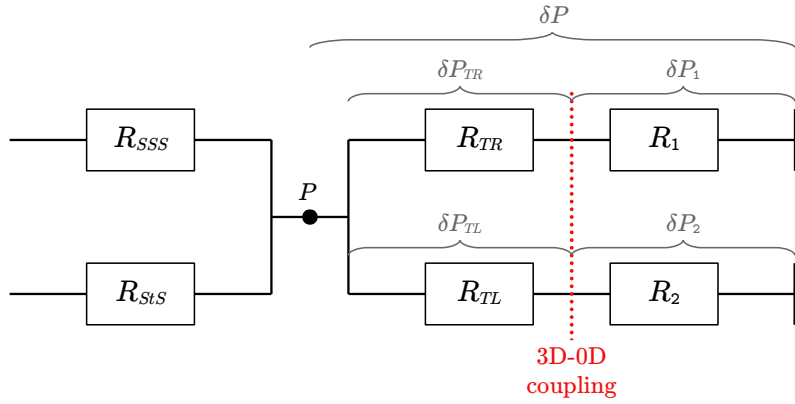
Figure 12: Model simplification.
