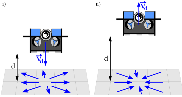
Figure 1: An expansion of the optic flow vector field is observed when a robot approaches a surface (i), while a contraction is observed when the robot moves away from it (ii).
