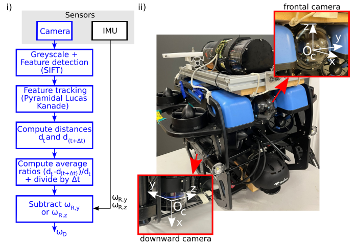
Fig. 2. i) Schema of the method used for measuring the optic flow divergence \omega_D . ii) The BlueBee robot is equipped with a frontal monocular camera and a downward monocular camera (with their respective coordinate systems \{O_c, \vec{x}, \vec{y}, \vec{z}\} ).
