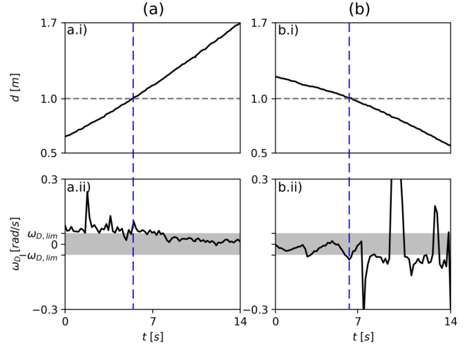
Fig. 6. Tests in which the BlueBee robot moves from the bottom of the pool to the surface (a) and descends from the surface to the bottom of the pool (b) respectively. (a.i and b.i) Distance d of the robot from the bottom of the pool given by the barometer. Only the time interval between 0s and 14s is shown, corresponding to the robot crossing the 1m threshold (dashed blue line). (a.ii and b.ii) Measured optic flow divergence \omega_D (in black) and area bounded by the thresholds \pm\omega_{D \lim} (in grey).
