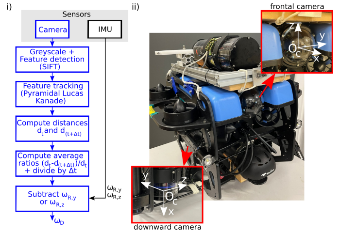
Fig. 2. i) Schema of the method used for measuring the optic flow divergence \omega_D . ii) The BlueBee robot is equipped with a frontal monocular camera and a downward monocular camera (with their respective coordinate systems \{O_c, \vec{x}, \vec{y}, \vec{z}\} ).
