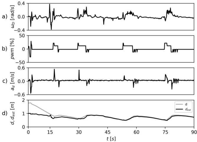
Fig. 4. Example of collision avoidance carried out in the ENSTA Bretagne pool (in Brest, Brittany, France): a) measured optic flow divergence \omega_D , b) pwm command given to the BlueBee robot, c) acceleration a_d in the direction of the obstacle given by the Inertial Measurement Unit (IMU) of the robot, d) comparison of the estimated relative distance d_{est} with the ground truth d given by the barometer. A video of the tests is available at https://youtu.be/qSBWyW11wX0 .
