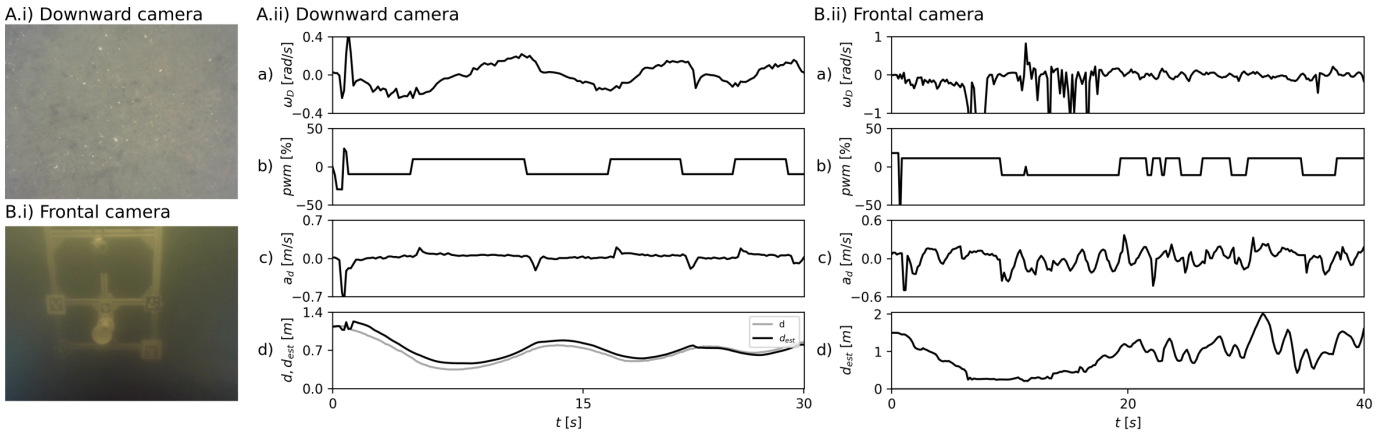
Fig. 5. A) Test carried out in the Moulin Blanc harbour (in Brest, Brittany, France): A.i) view from the downward camera, A.ii) a) measured optic flow divergence \omega_D , b) pwm command given to the robot, c) acceleration a_d in the direction of the obstacle given by the Inertial Measurement Unit (IMU) of the robot, d) comparison of the estimated relative distance d_{est} with the ground truth d given by the barometer. B) Test carried out in the Guerlédan lake (in Guerlédan, Brittany, France): A.i) view from the frontal camera, showing a hollow obstacle; A.ii) preliminary results. A video of the tests is available at https://youtu.be/qSBWYwI1wX0 .
