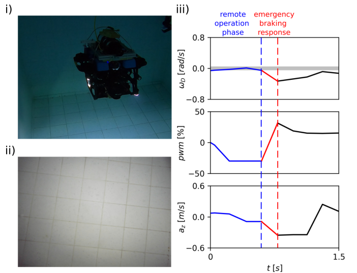
Fig. 3. i) The BlueBee robot in the ENSTA Bretagne pool (in Brest, Brittany, France). ii) View of the bottom of the pool from the downward camera. iii) Example of emergency braking response: the BlueBee robot was remotely controlled (in blue) until an optic flow divergence \omega_D below the threshold \omega_{D \text{ lim}} = -0.05 \text{ rad/s} (gray area) was measured and the autonomous emergency braking response was triggered (in red).
