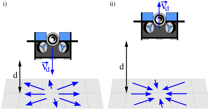
Fig. 1. An expansion of the optic flow vector field is observed when a robot approaches a surface (i), while a contraction is observed when the robot moves away from it (ii).
