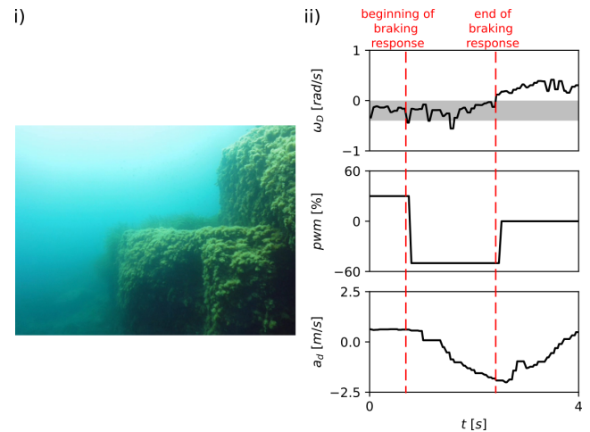
Figure 7: Test carried out in the Mediterranean sea (in Saint-Raphaël, Var, France): i) view from the frontal camera showing the obstacle, ii) preliminary results of emergency braking response. A video of the tests is available at https://youtu.be/qEFXrTL8Y2k .
