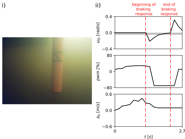
Figure 6: Test carried out in the Guerlédan lake (in Guerlédan, Brittany, France): i) view from the frontal camera showing an obstacle in the water column, ii) preliminary results of emergency braking response. A video of the tests is available at https://youtu.be/qEFXrTL8Y2k .
