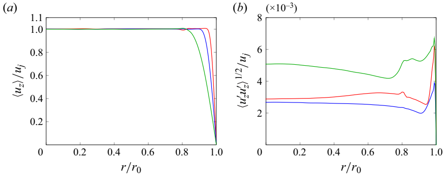
Figure 14. Nozzle-exit profiles of (a) mean and (b) r.m.s. axial velocity for M06BL05 (red), M06BL10 (blue) and M06BL20 (green).
