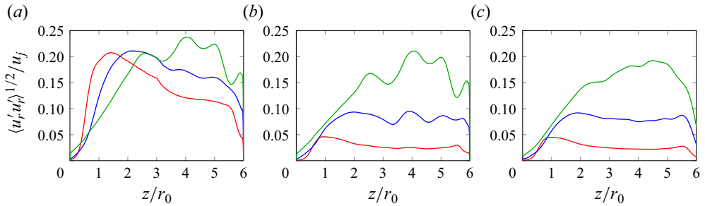
Figure 10. Variations of r.m.s. radial velocity fluctuations obtained for (a) the full signals, (b) n_\theta = 0 , and (c) the fluctuations of aerodynamic nature for n_\theta = 0 , at r = r_0 for M09BL05 (red), M09BL10 (blue) and M09BL20 (green).
