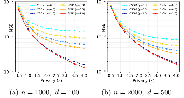
Figure 5: Mean Squared Error for CSGM and SIGM.
