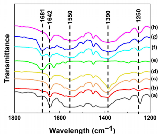
Figure 4. Fourier Transform infrared spectra of (a) anionic form of CA, (b) CL1, (c) CL2, (d) CL3, (e) CAD, (f) CLC1, (g) CLC2, and (h) CLC3.
