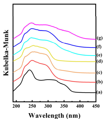
Figure 6. Solid-state diffuse reflectance spectra of (a) CA, (b) CL1, (c) CL2, (d) CL3, (e) CLC1, (f) CLC2, and (g) CLC3. For effective comparison, the peak maximums were normalized to have a similar value.
