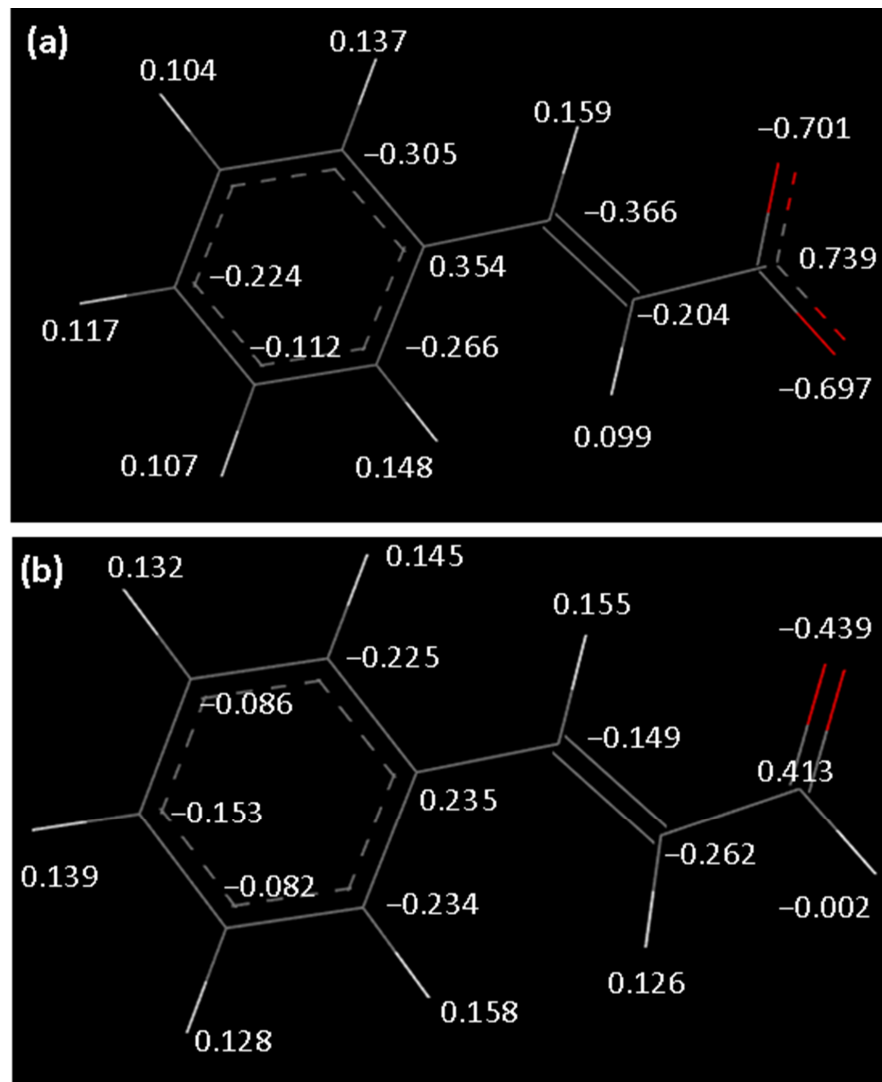
Figure 9. Partial charges extracted for DFT calculations for (a) CA ion and (b) CAD molecule.
