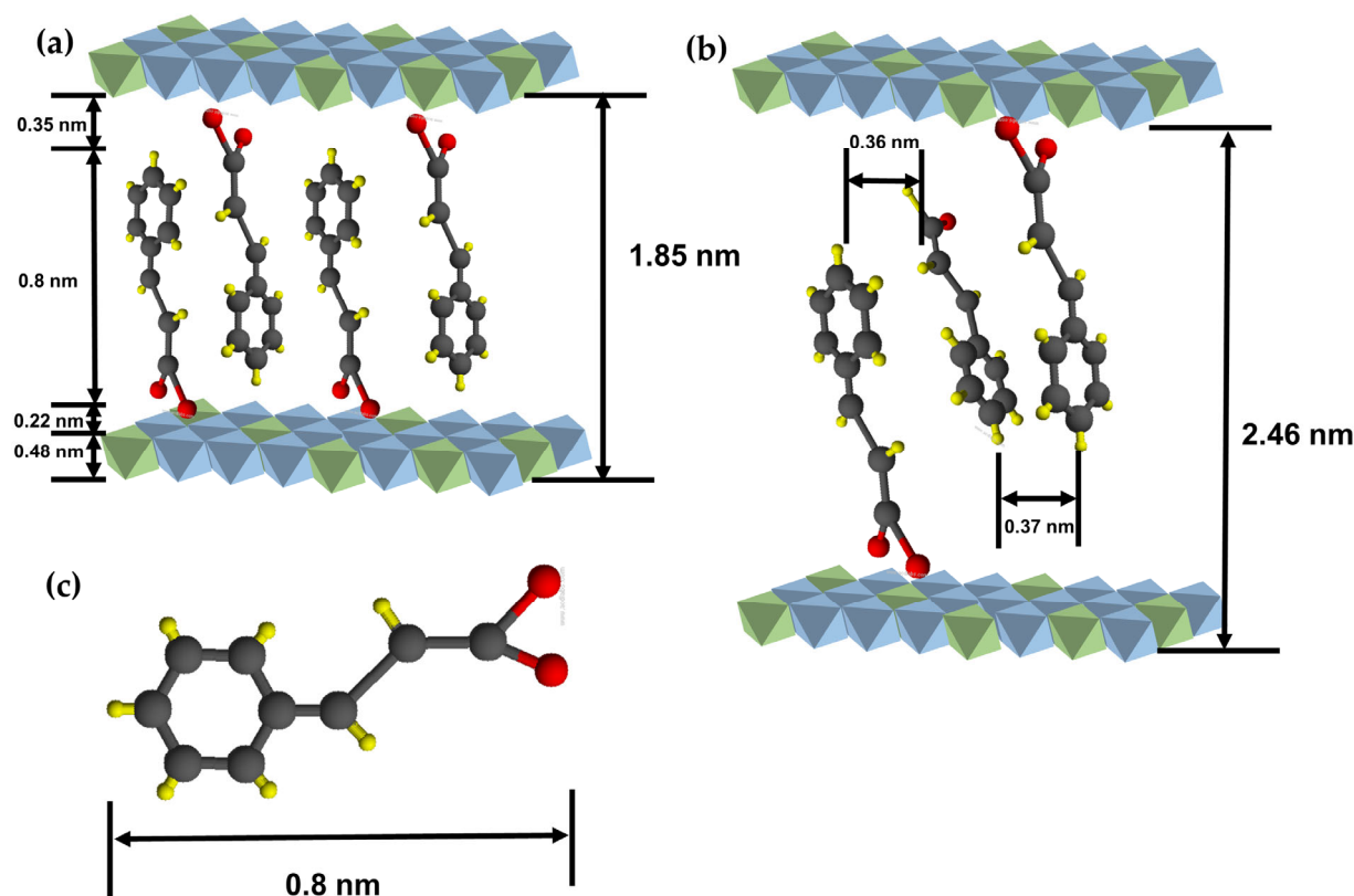
Figure 2. Schematic diagrams of interlayer molecular arrangements: (a) CL and (b) CLC. (c) Dimension of a cinnamic acid molecule. The color of atom representation is as follows: H (yellow), C (black), O (red), Al (green), Zn (blue).
