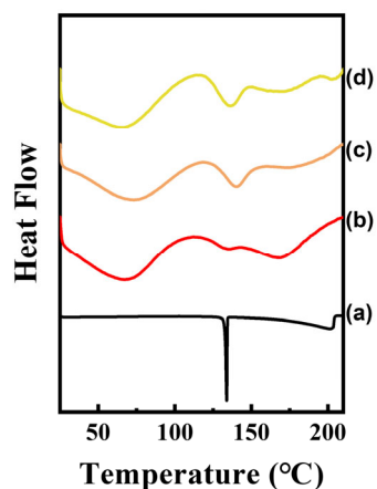
Figure 5. Differential scanning calorimetry (DSC) results for (a) CA, (b) CL1, (c) CL2, and (d) CL3. The DSC diagram was drawn with offsets to avoid overlapping curves.
