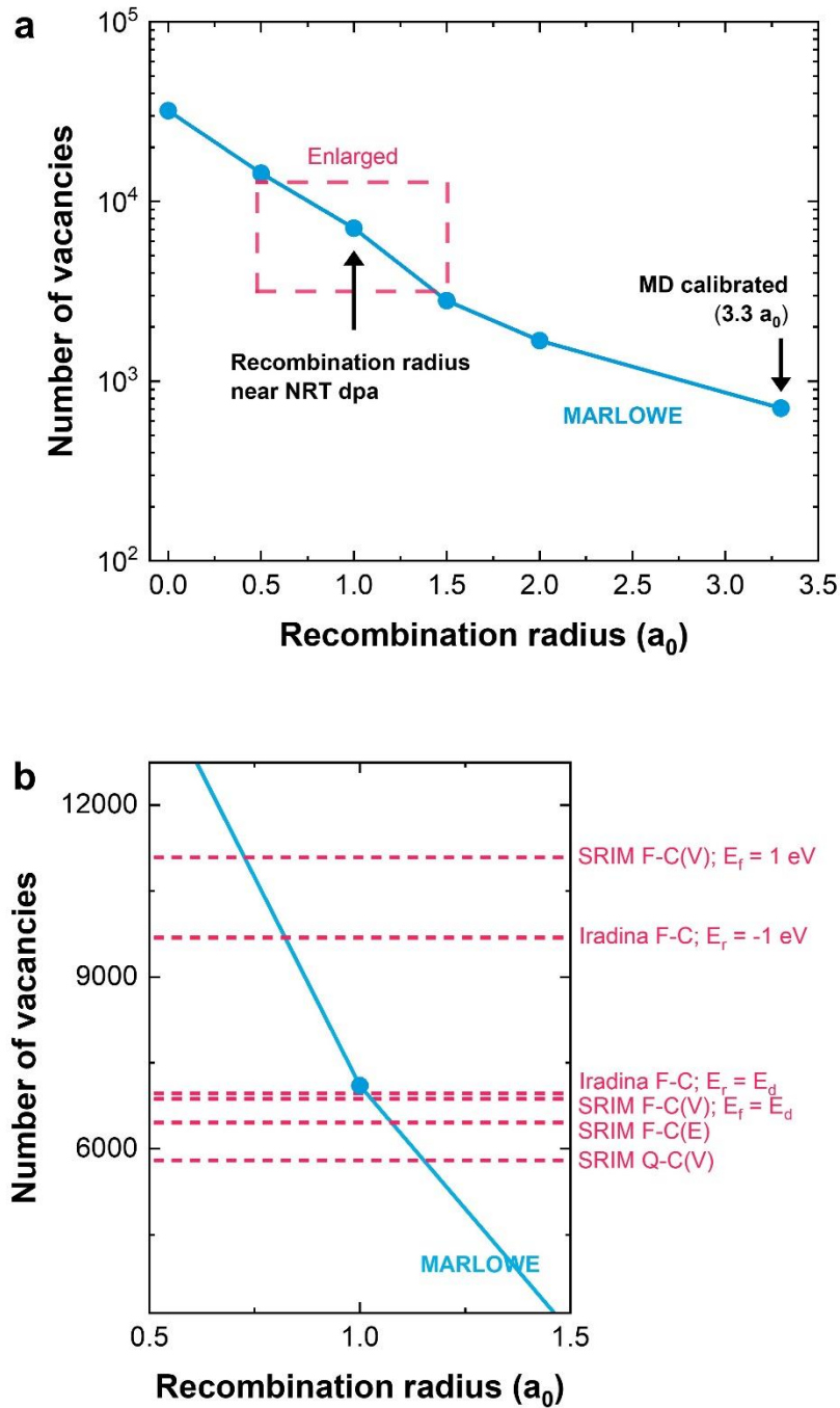
Fig 5. MARLOWE estimation of the number of vacancies as a function of recombination radius for 2 MeV self-ion irradiated Fe. The number of vacancies predicted by SRIM and Iradina with the same irradiation condition is indicated by the short lines. (F-C: full cascade option, Q-C: quick calculation option, “(V)”: vacancy.txt method, “(E)”: recoil damage energy method, E_f : final energy, E_r : replacement energy, E_d : displacement energy)
