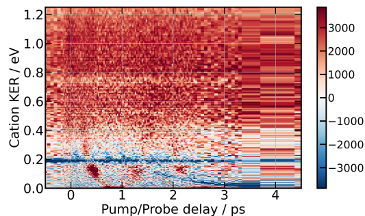
Fig. 11 266/334 nm experiment 3D-picture of S_2^{cation}(E, \tau) using the colour scale shown at the right hand side of the figure. Positive values indicate preferential dissociation along the polarisation direction of the pump laser.
