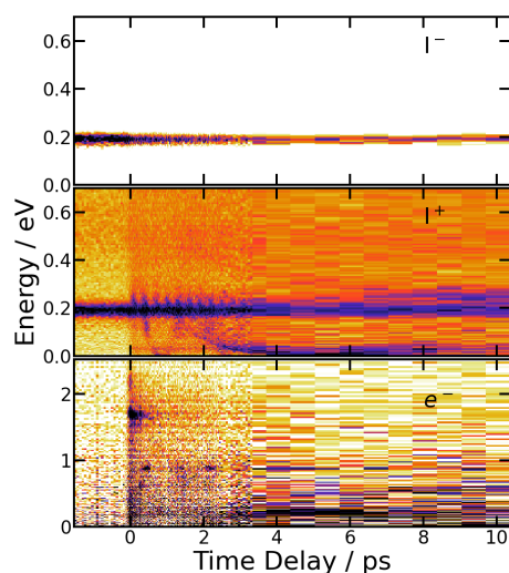
Fig. 9 266/334 nm experiment 3D-picture of S_0^{elec}(E, \tau) (bottom panel), S_0^{cation}(E, \tau) (middle panel) and S_0^{anion}(E, \tau) (top panel) using the same colour map as in Fig. 3.
