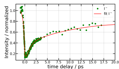
Fig. 4 269/807 nm experiment Sum of the S_0^{anion}(KER, \tau) fs-TRKERS for anion energies between 0.09 and 0.17 eV as a function of the pump-probe delay (green dots). The full red curve best fits the experimental signal as described in the text, using the time constants \tau^- , \tau_A and \tau_B listed in Tab. 1.
