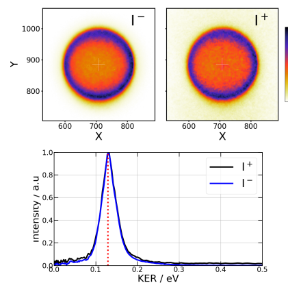
Fig. 2 Pump only experiment at 269\ \text{nm} Raw VMI images of I^- (top left panel) and I^+ (top right panel) and kinetic energy release (KER) (bottom panel) for each ion. The red dashed line in the bottom panel is the expected KER energy from energy conservation. The colour scale for intensities in the I^- and I^+ images is shown at the right hand side of the figure.
