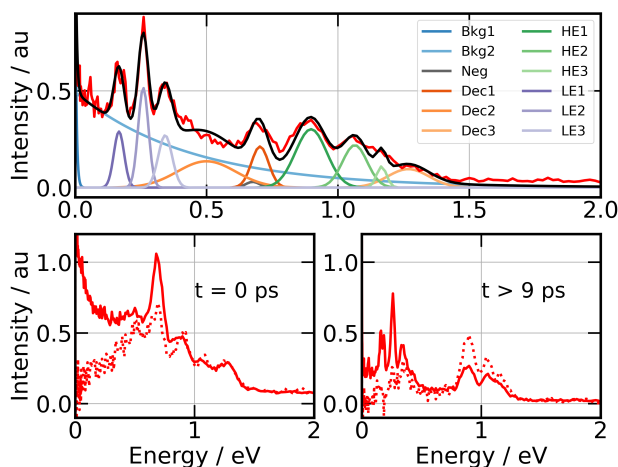
Fig. 8 269/807 nm experiment Top panel : Photoelectron spectrum obtained by projecting S_0^{elec}(KER, \tau) along the energy axis (vertical axis in Fig 7). Colours and labels isolate 9 bands, two continua and a further band for the signal at negative time. Bottom panels : Photoelectron spectra near \tau=0 ps (left panel) and above 9 ps (right panel) for isotropically distributed electrons (full line) and polarised electrons (dotted line). Both are obtained by integrating S_0^{elec}(KER, \tau) and S_2^{elec}(KER, \tau) over \tau , respectively, between -80 fs and +80 fs for the former, above 9 ps for the latter.
