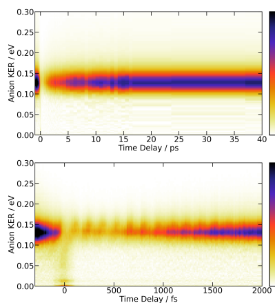
Fig. 3 269/807 nm experiment - 3D-plot of the fs-TRKERS signal S_0^{anion}(KER, \tau) , up to 40 ps (top panel) and 2 ps (bottom panel): the signal intensity is given by the colour map shown at the right hand side of the figure; it is plotted as a function of the I^- KER energy (vertical axis in eV) and pump-probe delay (horizontal axis).
