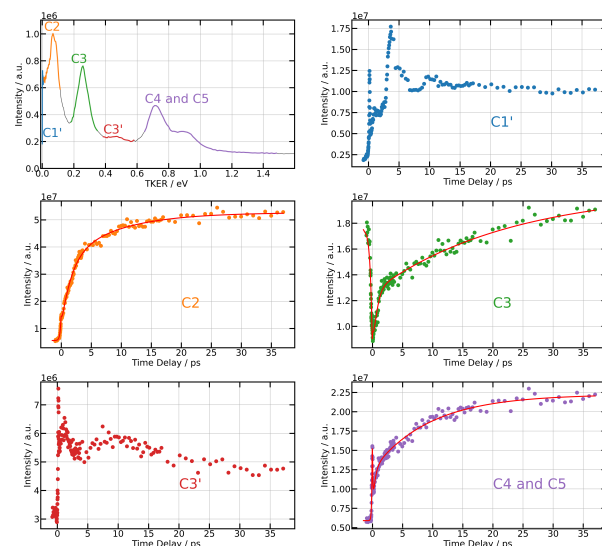
Fig. 6 269/807 nm experiment Top left panel : TKER spectrum obtained by integrating S_0^{cation}(KER, \tau) along the KER axis (vertical axis in Fig 5). The colours and labels C1', C2, C3, C3', C4 and C5 isolate 6 regions of interest (ROI). Note that TKER is twice the I^+ KER shown Fig.5. Other panels : time dependencies of the signal associated with each ROI. Dots show the experiment. Solid lines in ROIs C2, C3, and C4,5 are fit using the time constants listed in Tab.1.
