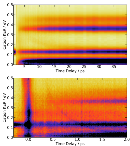
Fig. 5 269/807 nm experiment top panel : 3D-plot of the fs-TRKERS signal S_0^{cation}(KER, \tau) up to 40 ps time delay with the same colour map as in Fig. 3. Bottom panel : zoom on the first 2 ps with a different intensity scale to highlight the band whose central energy is changing with time delay. The top panel is reproduced on Fig. S6 of the ESI with another colour map that enhances the weak time-dependent feature described in the text. The equivalent 3D-plot of the fs-TRKERS signal S_2^{cation}(KER, \tau) are plotted on Fig. S7 of the ESI.
