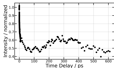
Fig. 10 266/334 nm experiment Total I^- anion signal as a function of the pump/probe time delay \tau , up to 600 ps (top panel) and 10 ps (bottom panel).
