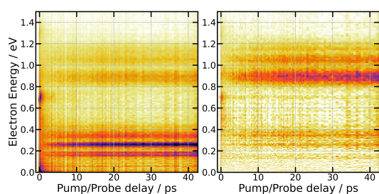
Fig. 7 269/807 nm experiment 3D-plot of the fs-TRPES signals S_0^{elec}(E, \tau) (left panel, isotropically distributed photoelectrons) and S_2^{elec}(E, \tau) (right panel, polarised electrons) with the same colour map as in Fig. 3.
