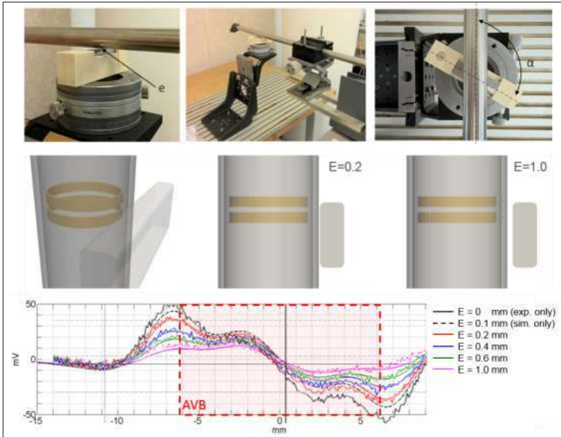
Figure 1. Quantitative comparison between simulated and experimental data with respect to the distance ( E ) between the AVB and the healthy tube: Experimental device (top), simulated configuration (center) and imaginary part of the impedance signal (bottom).
