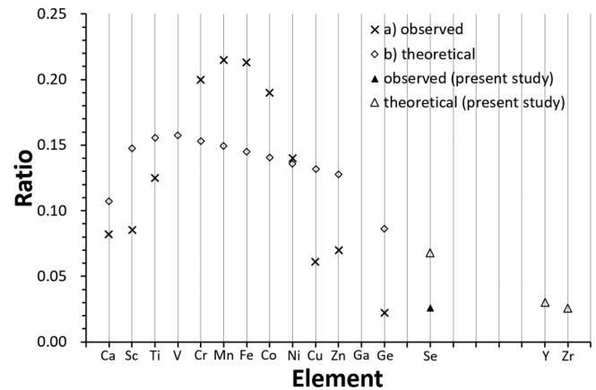
FIG. 9. Ratio of K\alpha_{12} satellite to the K\alpha_{11} diagram line intensities in Se is shown by a black triangle together with those of Refs. [20,48] marked by crosses (a). According to Ito et al. [20], this satellite is mainly considered to be a contribution of the [1s3d] shake process to the asymmetry of the K\alpha_1 emission line. Open rhombohedra (b) from Ref. [20] and open triangles from Table V represent the shake probability of [KM] , respectively. These values are based on the theoretical calculations. See the text in details.
