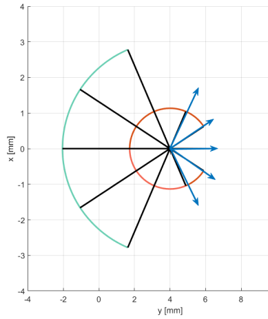
Figure 23. Top-view of the 2-tube CPPR ( \mathcal{R}_1 ) actuated in rotation only with \Delta\theta_d \in \{-\pi, -\pi/2, 0, \pi/2, \pi\} rad. The blue arrows represent one of the base vectors of the frame of reference attached to the tip of the CPPR and measured by the Aurora sensing device. The values of G_1 and G_2 are calibrated and the corresponding vectors of the model (black solid lines) are shown. See also Extension 7.
