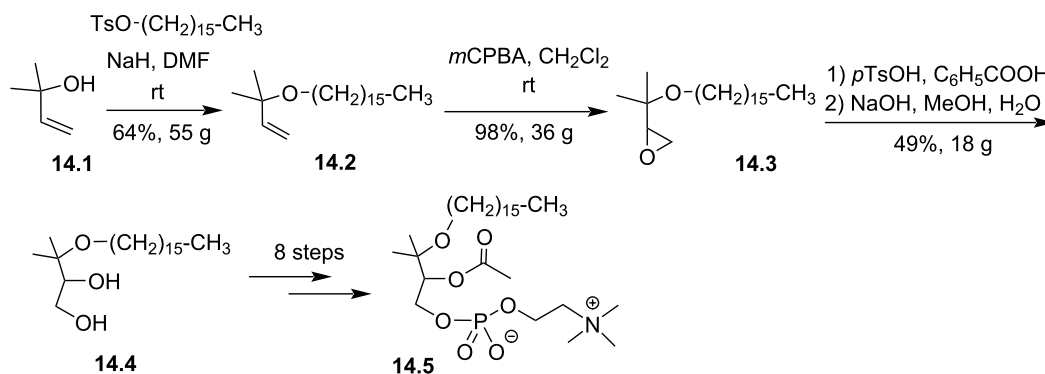
Figure 14: Racemic synthesis of 14.5 as an illustration of the introduction of methyl substituents on the glycerol backbone of PAF [97].
