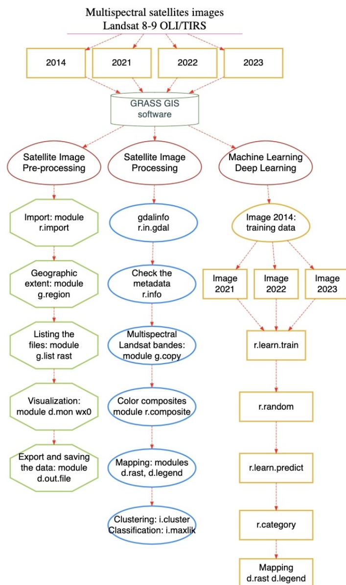
Figure 3. Workflow scheme illustrating the methodology used in this study for image processing by GRASS GIS. Software: R version 4.3.3, library DiagrammeR version 1.0.11 [95]. Diagram source: author.
