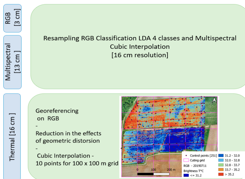
Figure 5. Map of the re-sampling of the 11 July 2019 thermal image.
