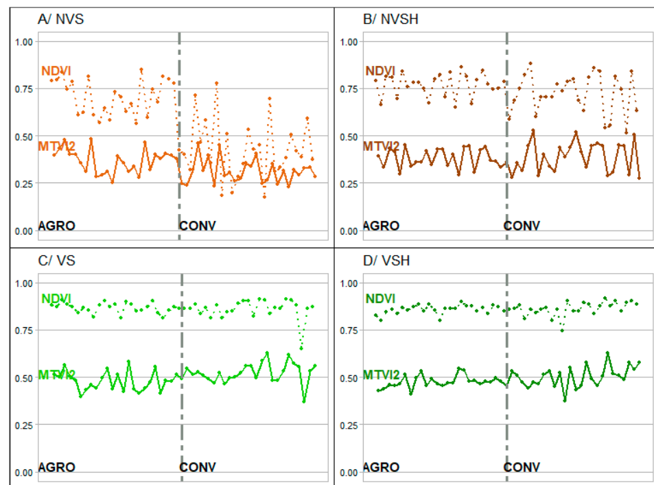
Figure 11. Values of the NDVI (dotted line) and MTVI2 (solid line) indices for NVS, NVSH, VS, VSH classes—25 AGRO points followed by 25 CONV points.
