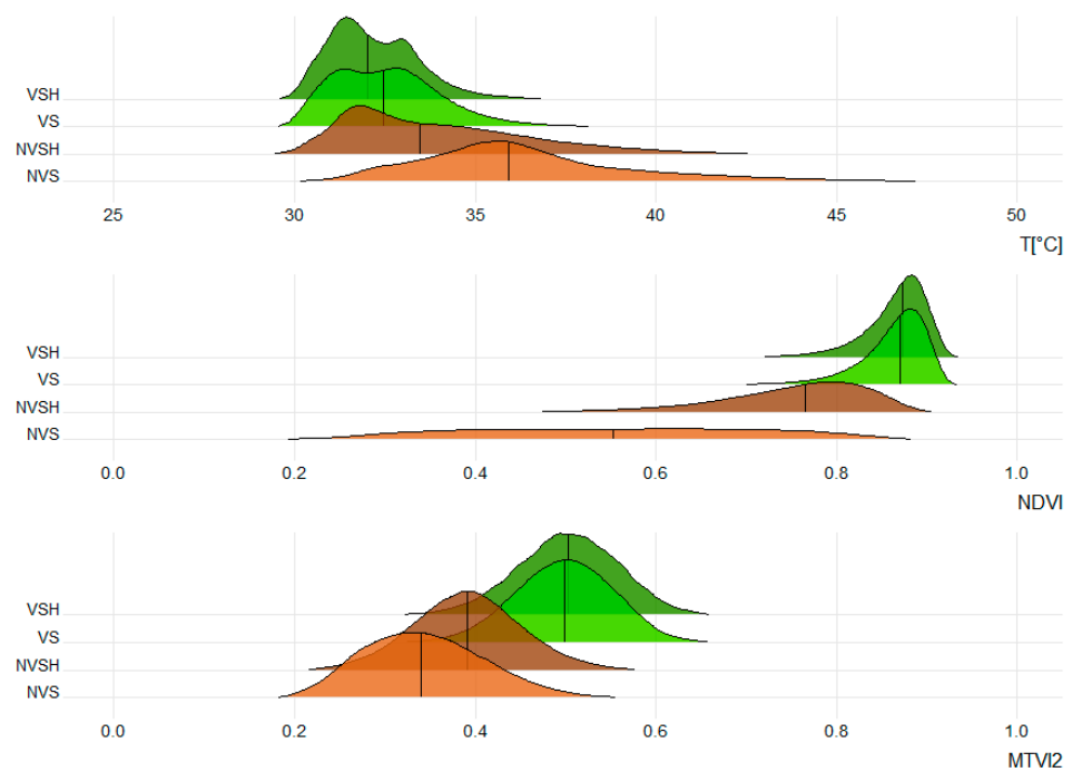
Figure 8. Comparison of temperature values at 12:49 pm and various indices for each land-use class (NVS light brown, NVSH dark brown, VS light green, VSH dark green).
