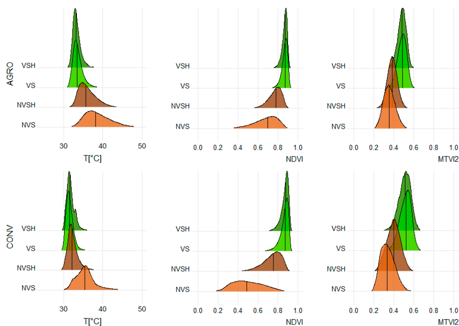
Figure 10. Comparison of the temperature values at 12:49 p.m., of the indices and of the land use class (NVS light brown, NVSH dark brown, VS light green, VSH dark green) between both plots.
