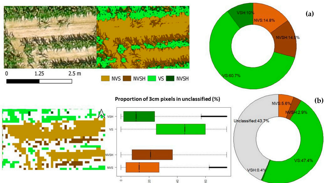
Figure 4. From left to right: (a) RGB image of the 11 July 2019; Original classification at 3 cm resolution and Proportion [%] of the different classes of land cover before re-sampling. (b) Classification after re-sampling at 16 cm, Proportion [%] of the different classes of land cover that did not meet the 75% purity criterion, Proportion [%] of the different land cover classes of 75% purity and above.
