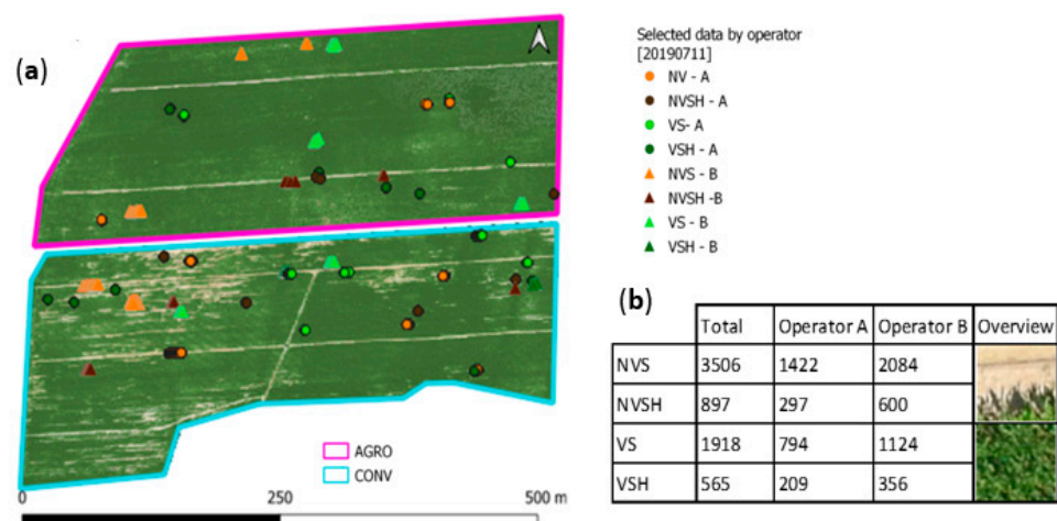
Figure 2. (a) Positioning of sample class types by operators (A or B) on the UAV image of the 11 July 2019. (b) Frequency of sampling points according to land use type and operator (11 July 2019).
