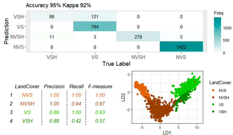
Figure 6. Classification performance measurements using the twelve primitives selected for the 11 July 2019 image and positioning of the samples on the first two linear discriminants (LD1 and LD2).
