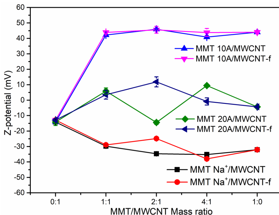
Figure 1. \zeta -potential of various combinations of MMT/MWCNT.
