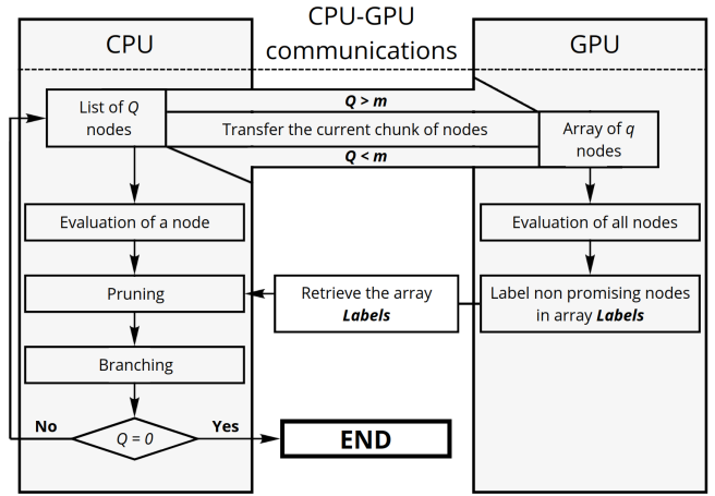
Figure 3: Flowchart of the proposed GPU-accelerated tree-search algorithm.
