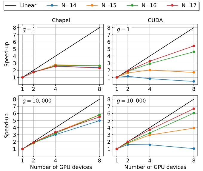
Figure 7: Speed-up achieved by our Chapel implementation compared to the CUDA-based implementation executed on the Nvidia V100 GPUs. Results are shown for different instances and granularities.
