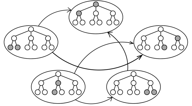
Figure 1: Illustration of the parallel tree-exploration model.
