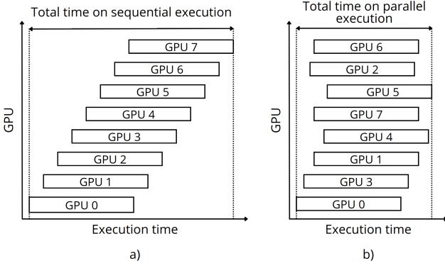
Figure 4: Approaches for launching many GPUs (kernels): a) sequential version; b) parallel version using multi-threading.
