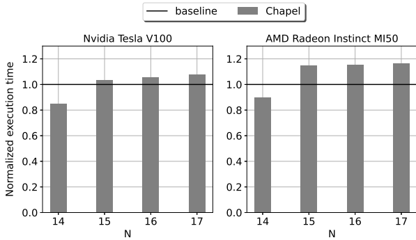
Figure 6: Normalized execution time of the Chapel implementation compared to the CUDA and HIP baselines on the Nvidia V100 and AMD MI50 GPU architectures, respectively.
