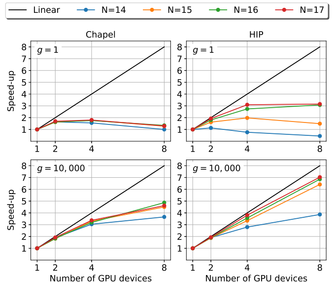
Figure 8: Speed-up achieved by our Chapel implementation compared to the HIP-based implementation executed on the AMD MI50 GPUs. Results are shown for different instances and granularities.
