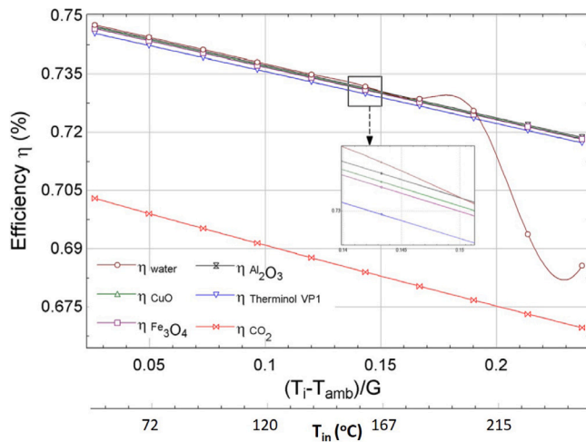
Fig. 12. Thermal efficiency comparison for six different working fluids. Pressurized water, Therminol VP-1, \text{CO}_2 , and three oil-based nanofluids with 3 vol% of \text{CuO} , \text{Fe}_3\text{O}_4 , \text{Al}_2\text{O}_3 dispersed in Therminol VP-1.
