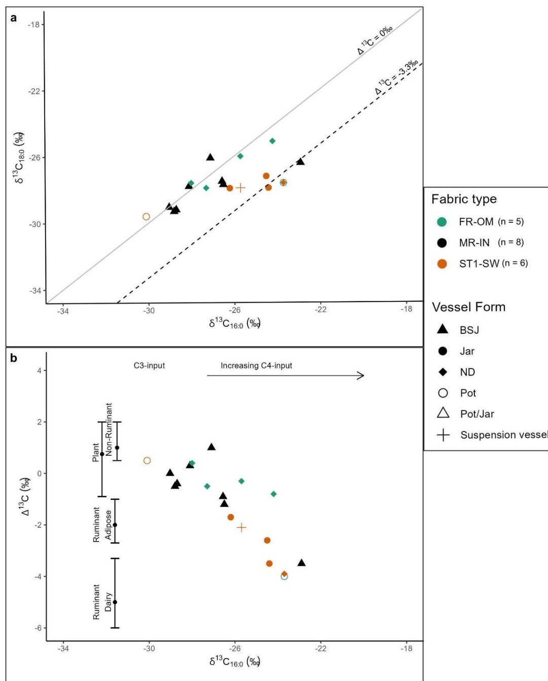
Figure 6: Scatter plots showing the \delta^{13}\text{C} values of (a) \text{C}_{18:0} and \text{C}_{16:0} fatty acids and (b) \Delta^{13}\text{C} ( \text{C}_{18:0} – \text{C}_{16:0} ) and \text{C}_{16:0} fatty acid values, measured from lipid extracts of potsherds from Salūt-ST1. In (a), the dashed line at -3.3\text{‰} indicates the limit of \Delta^{13}\text{C} values for reference dairy fats and the grey line indicates 0\text{‰} . In (b), ranges depicted represent the mean \pm 1 s.d. of \Delta^{13}\text{C} values of modern reference terrestrial fats from Africa and Asia and \text{C}_3 plant oil references published elsewhere (Craig et al., 2005; Dunne et al., 2012; Lucquin et al., 2016; Outram et al., 2009; Steele et al., 2010). Modern references from the study region are not yet available. Instrumental error is less than \pm 0.5\text{‰} . BSJ, Black Slipped Jar; FR-OM, Fine Red Omani Ware; ND, vessel form not determined; ST1-SW, ST1 Sandy Ware.
