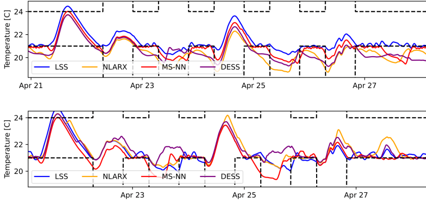
Fig. 3: Experimental results for the typical heat day scenario using a dynamic price signal. The upper graph represents results with the restricted dataset, and the lower one represents those using the extended dataset.
