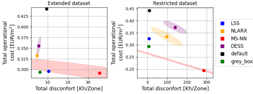
Fig. 1: BOPTEST KPI obtained with selected models using the extended and restricted dataset. Variance estimated using the five different trainings. Score computed with the scenario typical heat day and dynamic price signal.
