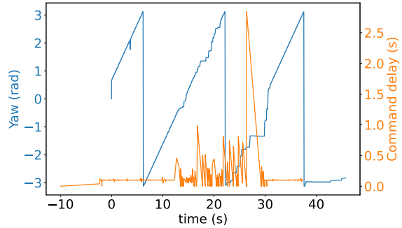
Fig. 3: Yaw value (in blue) with corresponding command delays (in orange) for one experimental run with the experimental configuration S_5 with perturbation between t=15s and t=30s .
