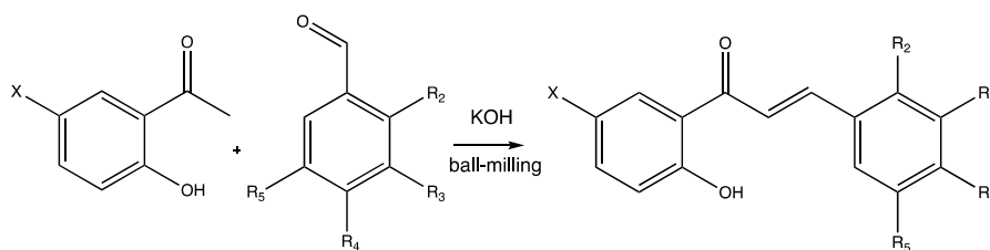
Figure 3. Reaction of chalcones synthesis under ball milling conditions.
