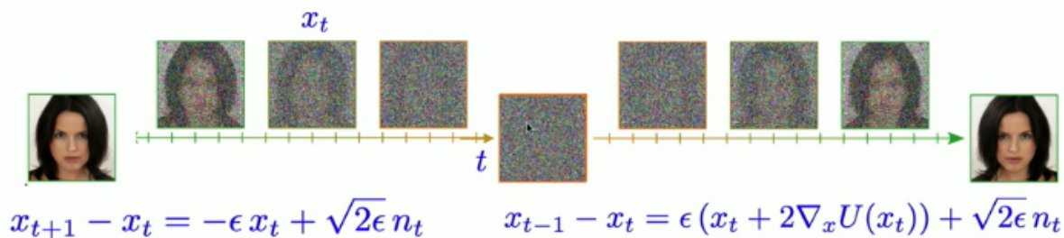
FIGURE 7 – Example of the evolution of an image by the stochastic process of a diffusion model: on the left, a progression where noise is injected (forward) and on the right, where denoising is carried out
