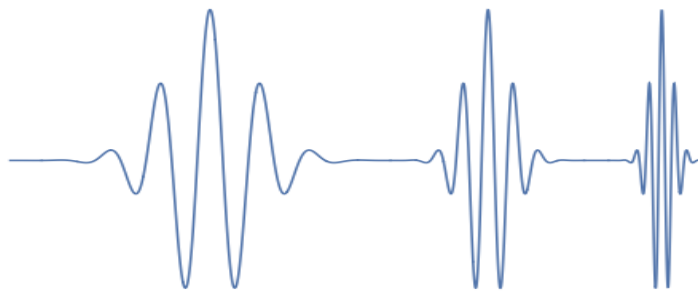
FIGURE 32 – Illustration of translation and scaling operations applied to a wavelet.
