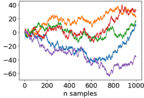
FIGURE 20 – 1D Random Walk: X_n = X_{n-1} + Z_n where Z_n follows a Bernoulli distribution \{+1, -1\} ( p(+1) = 1/2 ). All five chains start at the origin x_1 = 0 . See the notebook randomwalk.ipynb .
