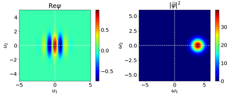
FIGURE 37 – Basic 2D wavelet (Eq. 310) with its Fourier spectrum localized around \omega_1 \approx \xi ( \sigma = 1 , \xi = 5/4\pi ), with zero power in the \omega_1 \leq 0 plane.
