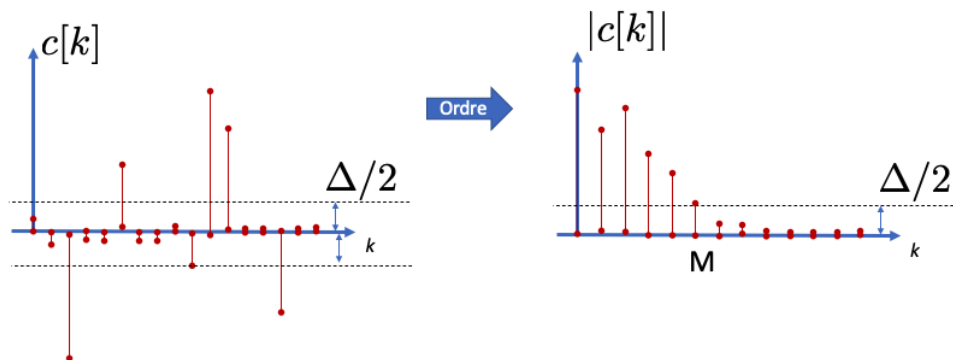
FIGURE 37 – Illustration of sorting coefficients c[k] and the relationship between the number of coefficients M and the threshold \Delta/2 .
