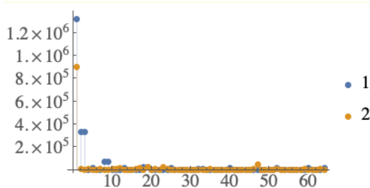
FIGURE 30 – The squared magnitude values of the 64 coefficients in the decomposition of the two images in Figure 28: "1" corresponds to the image with a discontinuity, and "2" is for the random image.
