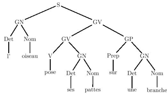
FIGURE 19 – Analysis through a syntax tree of the sentence: "l'oiseau pose ses pattes sur une branche" ("The bird puts its paws on a branch").
