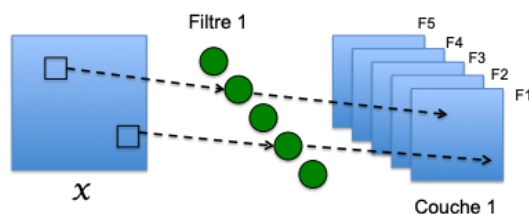
FIGURE 6 – Schematic of a first convolutional layer with 5 different filters. For each filter, e.g., filter F1, each neuron handles a small part of the original image, and all weights associated with each neuron are identical across neurons.
