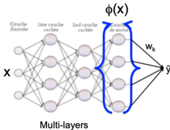
FIGURE 5 – Simplified diagram of a multi-layer neural network where the representation \Phi is the result of all the sub-layers; it is used at the end of the network for tasks such as classification.
