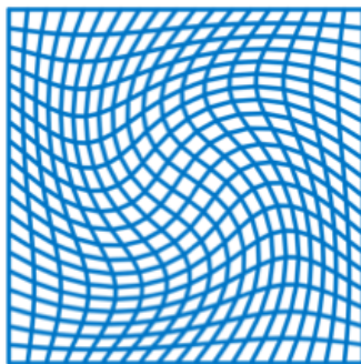
FIGURE 31 – Example of a diffeomorphism applied to a square.
