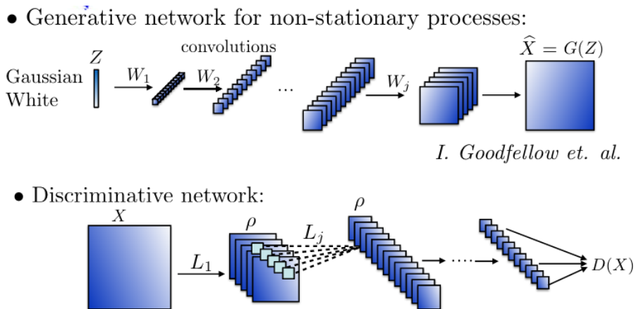
FIGURE 22 – Schematic architecture of Generative Adversarial Networks.
