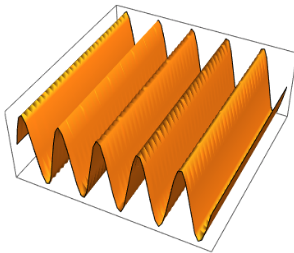
FIGURE 46 – Ridge sinusoidal function varying in only one dimension.
