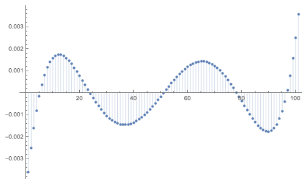
FIGURE 45 – Residuals of fitting the function x^5 with a degree 4 polynomial.
