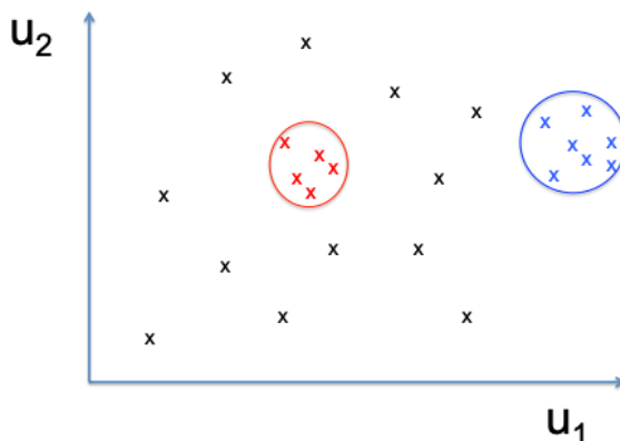
FIGURE 32 – Illustration of short-distance interactions within a group.
