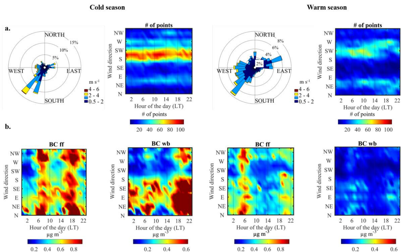
225 Figure 1: Wind analysis and BC ff and BC wb levels at the ATOLL site during the cold (left, Sep-Apr) and warm (right, May-Aug) seasons. a) Wind roses and wind frequency by the hour of the day (minimum wind speed of 0.5 m s -1 ). b) Contour plots of BC component loadings according to the wind sector and hour of the day. The color scale minimum and maximum values in (b) correspond to the 5 th and 75 th percentiles for each season, respectively.
