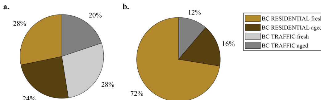
385 Figure 6: Relative contributions from residential and traffic emitted less than 24 hrs (fresh) and more than 24hrs (aged) before reaching the ATOLL site: (a) the mass loading of BC; (b) the light absorption coefficient of BrC calculated at 470 nm.
