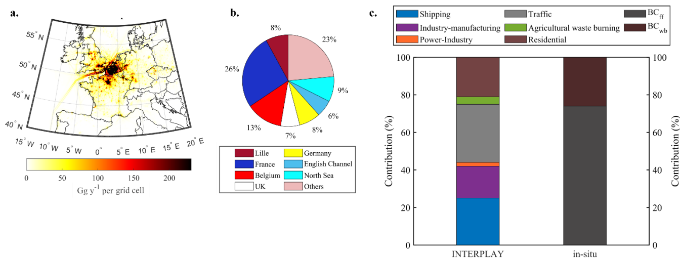
255 Figure 2: (a) Spatial contribution of BC to ATOLL in Gg\ y^{-1} per grid cell and its (b) relative contribution by region/country; (c) sectorial distributions according to INTERPLAY and in-situ via the aethalometer model. Results over the period Dec 2016 – Dec 2019.
