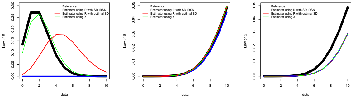
Figure 1: Results for the Signal distribution estimators of \mathcal{P}(\theta) using X , R irsn and R opt for n = 50, N = 5 for high values of C_{bl} and C_{gr} for model a) (left) b) (center) and c) (right).
