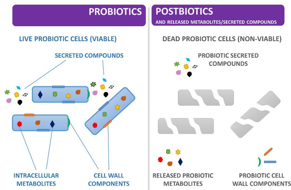
Figure 2. Graphic schematisation of the concepts of probiotic (on the left), postbiotic and released metabolites/secreted compounds (on the right). This review focuses on L. plantarum secreted compounds (i.e., CFS or isolated compounds from CFS) with antimicrobial activity.
