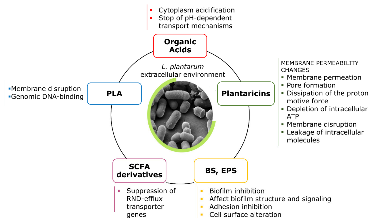
Figure 3. Different chemical nature of the principal antimicrobial agents produced by L. plantarum strains, and the suggested mechanisms underlying their antimicrobial effect. PLA: phenyl lactic acid; SCFA: short-chain fatty acids; BS: biosurfactants; EPS: exopolysaccharides.
