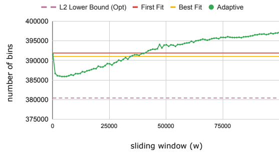
(b) GI benchmark from BPPLIB.
