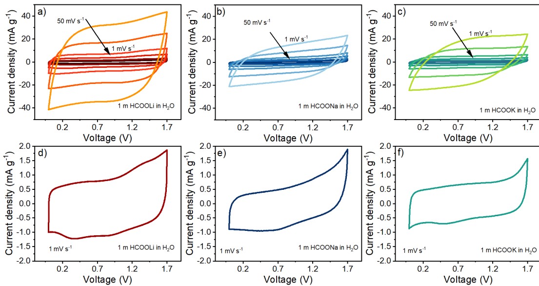
Figure 3. CV of the cells containing a) and d) 1 m HCOOLi in \text{H}_2\text{O} ; b) and e) 1 m HCOONa in \text{H}_2\text{O} ; c) and f) 1 m HCOOK in \text{H}_2\text{O} CV at scan rates of 1 \text{ mV s}^{-1} , 2 \text{ mV s}^{-1} , 5 \text{ mV s}^{-1} , 10 \text{ mV s}^{-1} , 20 \text{ mV s}^{-1} and 50 \text{ mV s}^{-1} .
