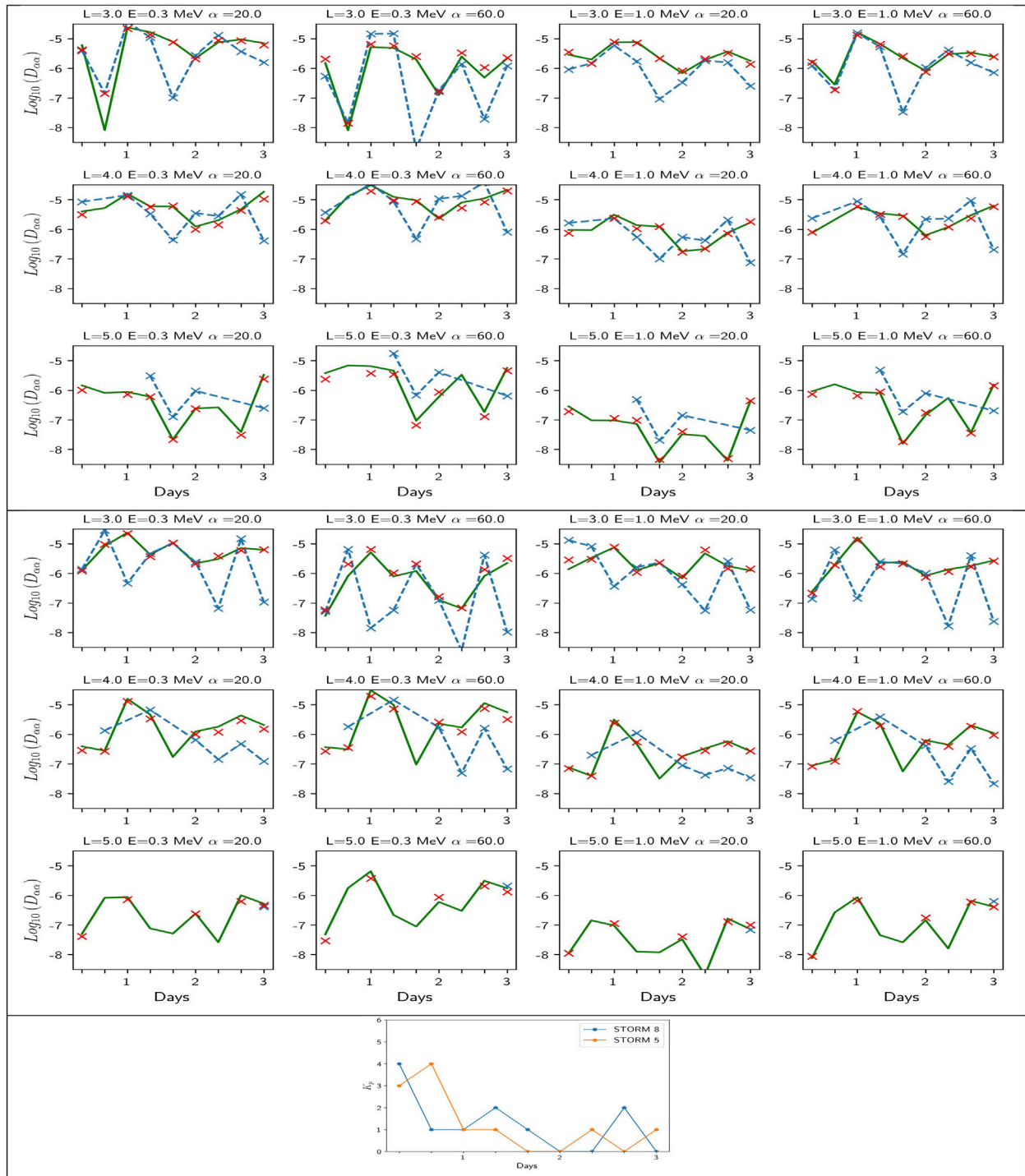
FIGURE 5 | Pitch angle diffusion coefficients for (1–3 rows) storms 8 and (4–6 rows) storm 5. The first 6 panels show historic pitch-angle diffusion coefficient's at different ( L , E , \alpha ) values, with (blue crosses and lines) the raw data of event-driven coefficients (red crosses) the averaged data (on the 32 storms at given ( K_p , t , L , E , \alpha )), and (green lines) the DNN model. The average data (in red) and the DNN model (in green) (trained on a subset of the average model) are run from the K_p(t) sequence of each storm plotted at the bottom panel for each of the 9 temporal bins. The good agreement between red crosses and the green line shows the success of the DNN model at matching its target. Both capture levels and variations, but are not very accurate compared with the event-driven diffusion reference values in blue, showing the limits of a mean model.
