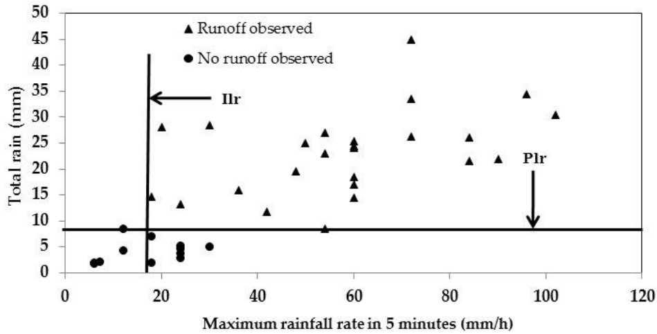
Fig. 4 Example of determination of the rain ( Plr ) and threshold intensity ( Iir ) of runoff on the plot S_{1-150\text{ m}^2} for the year 2010
