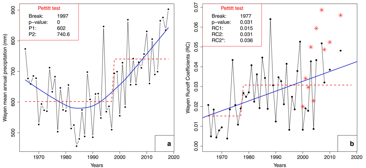
Fig. 7. Evolution of annual precipitation (a) and runoff coefficient (b) in Nakanbé watershed at Wayen. Blue curve/line shows the trend and red dashed lines, the breakpoints. Red stars represent the reconstituted runoff coefficient (RC2*) after the impoundment of Ziga and Dourou dams, P1/RC1 refers to the period before breakpoint and P2/RC2 refers to the period after breakpoint. P designated precipitation and RC runoff coefficient.
