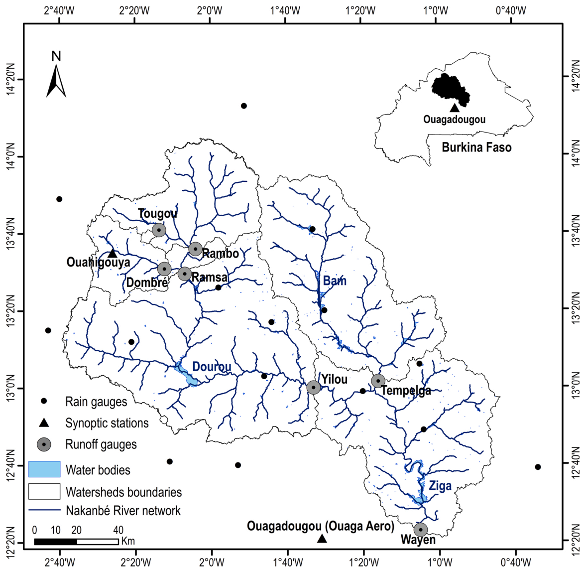
Fig. 1. The Nakanbé nested watersheds at Wayen (38 - 21,178 km 2 ), located in the West Africa Sahel, with drainage network, water bodies, available rain gauges, synoptic stations and runoff gauges.
