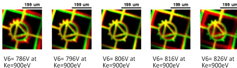
FIGURE 3 Effect of the magnification objective lens V6 at 900 eV on a gold grid sample image. The red image color corresponds to the grid image at KE = 900 eV and the green image is the image formed for KE = 1,402 eV representing the reference image against which changes to V6 voltage are compared. Yellow is obtained for pixels where the overlay of the red and green are of equal intensity in the respective color scales.
