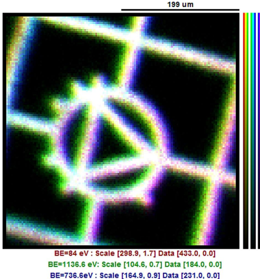
FIGURE 1 Overlay of gold grid measured at different binding energy using a monochromatic Al K alpha source. The white color corresponds to a perfect overlay of these 3 images. The measure was performed with a Kratos Nova instrument at PE 160 eV.
