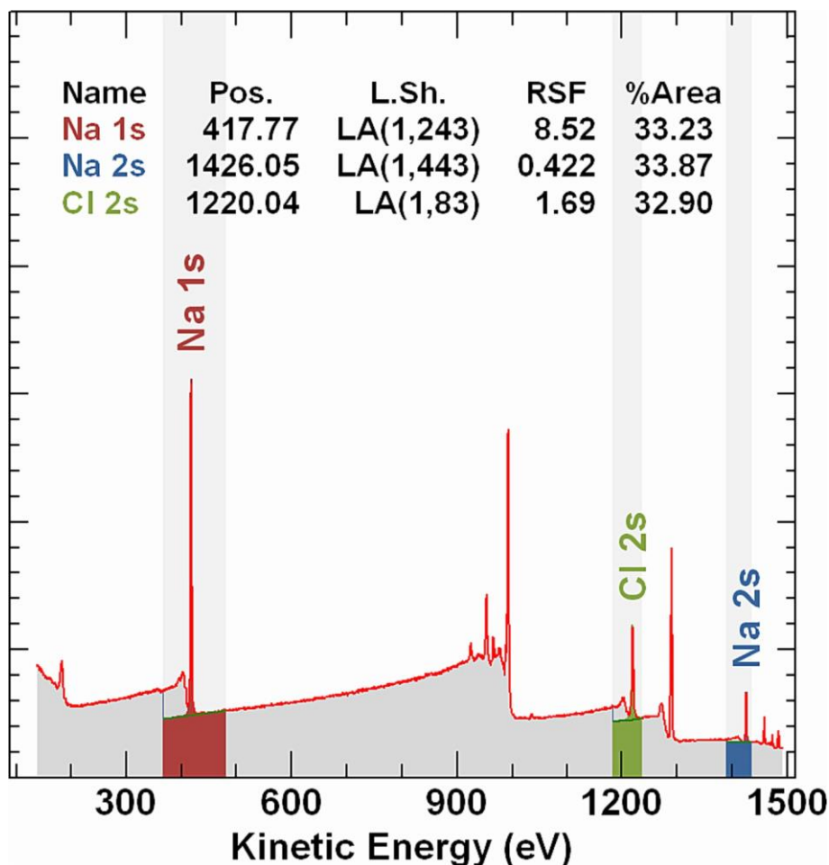
FIGURE 10 Quantification of Axis Nova FoV2 PE 160 spectrum measured from NaCl crystal. Photoemission intensities are measured by making use of Voigt line shapes and backgrounds extrapolated from signals with higher kinetic energy that the photoemission peak corresponds to Na 1s, Cl 2s, and Na 2s. Scofield cross-sections were corrected for effective attenuation length escape depth correction and no transmission correction.
