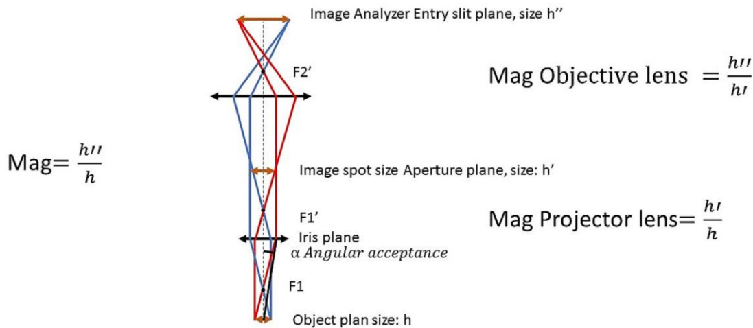
FIGURE 2 Diagram of the lens column for both Kratos Axis Ultra and Kratos Axis Nova.
