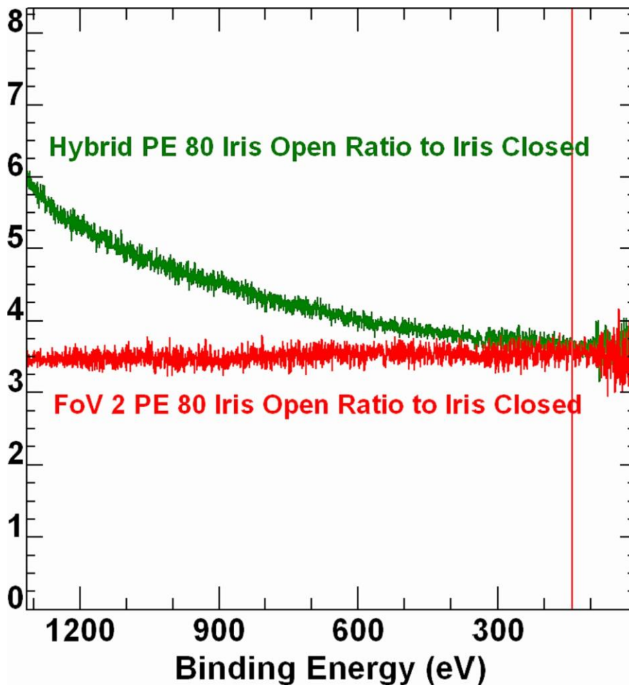
FIGURE 9 Axis Ultra gold spectrum was measured using PE 80 hybrid and PE 80 FoV 2 measured using angular-acceptance iris fully open and fully closed. Spectra are displayed relative to the iris closed position for angular acceptance concerning each operating mode. Note FoV 2 shape is identical for angular acceptance iris open and closed. Closing the iris simply reduces sensitivity.
