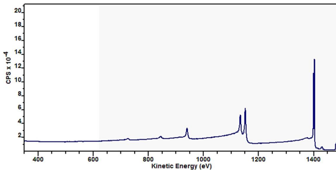
FIGURE 5 True gold spectrum between kinetic energy 350 and 1,492 eV with a step of 0.4 using an FOV2 with a surface analyzed of 150 \mu\text{m} by 500 \mu\text{m} PE 160 eV.
