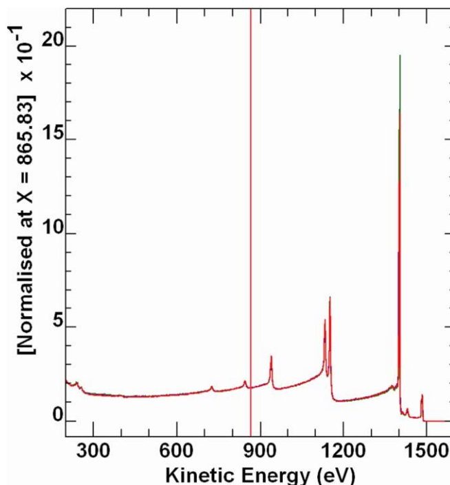
FIGURE 7 Gold survey spectra measured from the clean gold sample. Three spectra are overlaid including NPL transmission corrected Axis Ultra hybrid mode PE 80 eV from John Walton, 11 Axis Nova FoV2 PE 160 eV, and FoV2 PE 80 eV.
