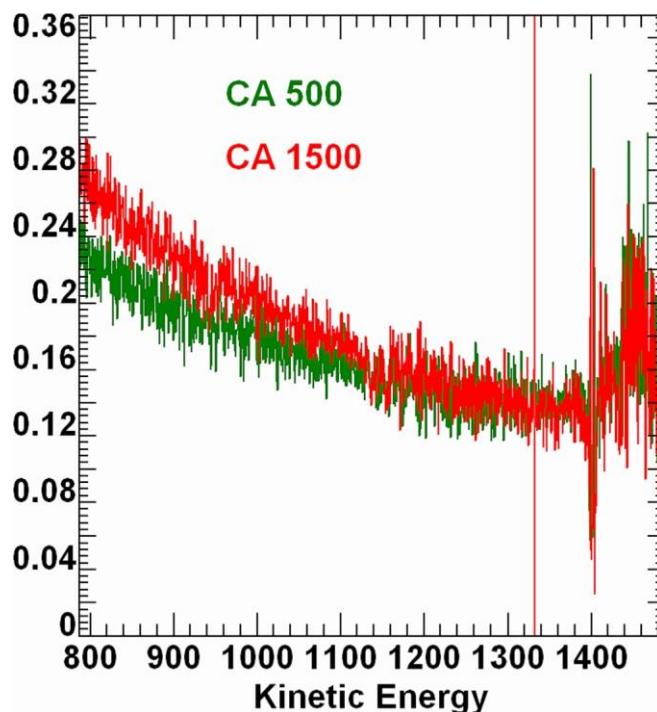
FIGURE 8 NanoESCA clean gold sample spectra relative to NPL true gold spectrum. Transmission for PE 50 CA 500 obeys an energy law of E^{-0.9} while CA 1500 obeys E^{-1.25} .
