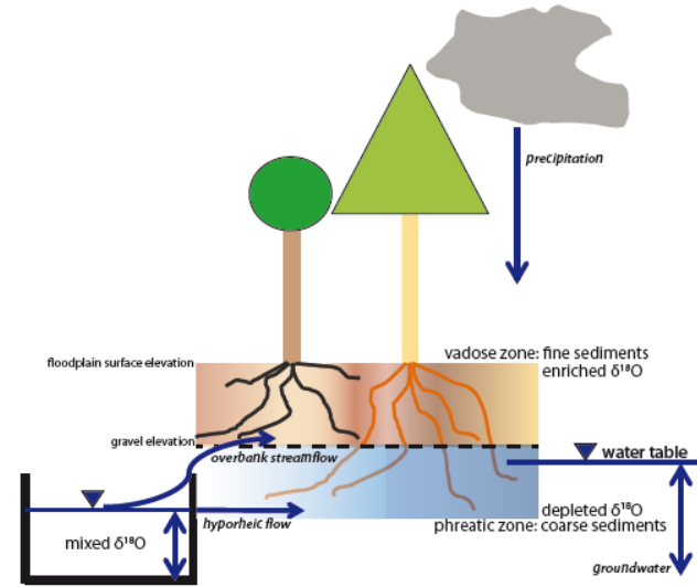
Figure 1 -Schematic showing how two species with contrasting rooting depths may record different annual values of \delta^{18}\text{O} based on variability in hydrologic partitioning between floodplain storage reservoirs. There is a large dependence on the depth to gravel and the relative surface elevation of the floodplain above the water table.
