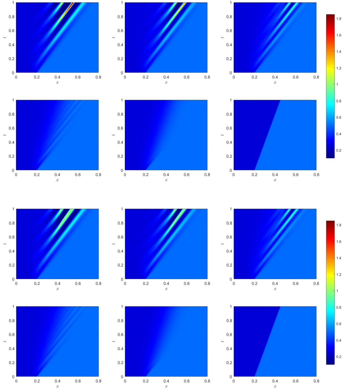
Figure 7: Two top rows: Keimer and Pflug's delayed model (1.2), \tau = 0.1, 0.08, 0.06, 0.04, 0.02 (as in [14, Figure 3]); Two bottom rows: delayed model (1.1), same \tau and exponential saturation function. The lower rightmost figure in both the couples of rows is the solution to the LWR model with initial datum (5.11). For the other graphs, we fix L = 0.1 and linear decreasing kernel.
