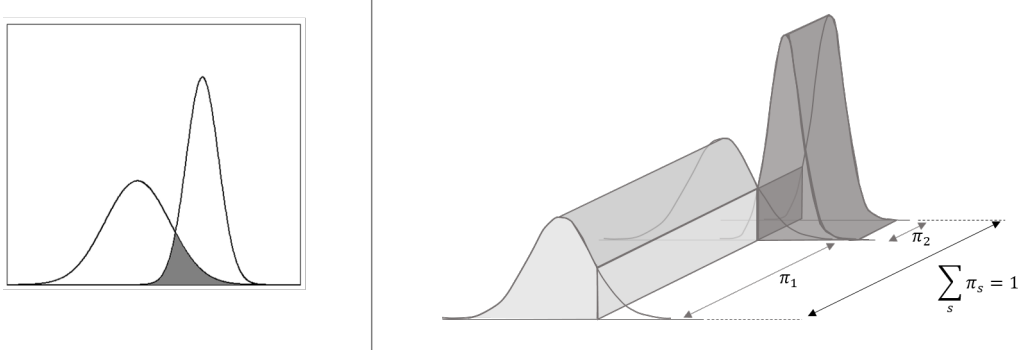
Figure 2. Overlap between PDFs and accuracy of state decoding assuming a simple mixture model with one single state-dependent variable. Each PDF is Gaussian. Knowing the variable value, the probability of getting the correct state corresponds to the PDF that is maximum weighted by the probability of being in the corresponding state.
