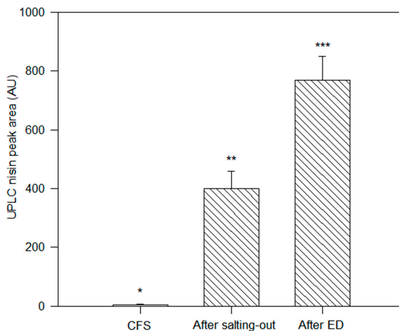
Figure 4. UPLC peak area of nisin in the initial CFS, after salting out and after ED purification. Nisin peak was confirmed by MS according to its 3500 Da molecular weight. Columns with a different number of asterisks (*) are significantly different at p < 0.05 ( t -test).
