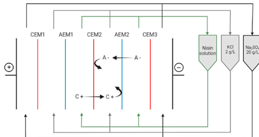
Figure 2. Configuration of the electro dialysis cell. CEM: cation exchange membrane; AEM: anion exchange membrane. C+: cations, A−: anions.
