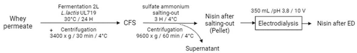
Figure 1. Flowchart of nisin production and purification from a cell-free supernatant (CFS) using ammonium sulfate salting out and electro dialysis (ED).
